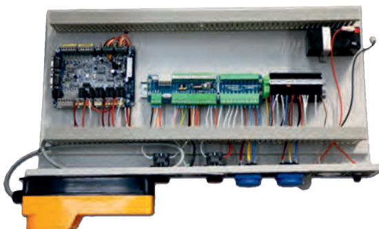
MAINTENANCE BOX
